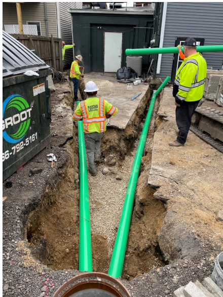
Downspout Construction
