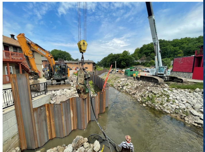
Cofferdam Construction
